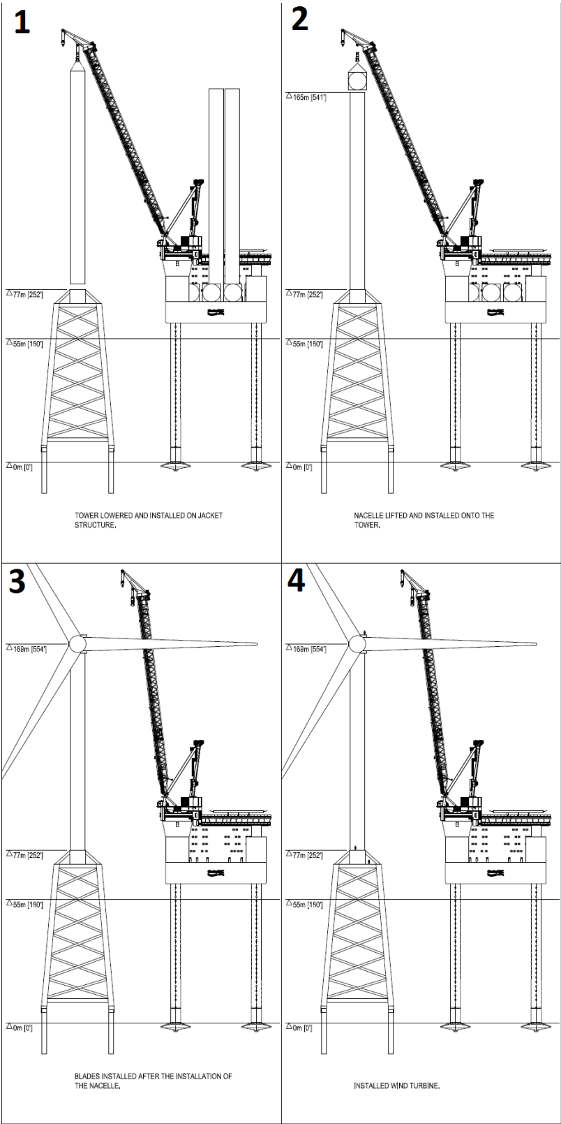
Figure 8. Campaign 3 Turbine Installation Sequence
